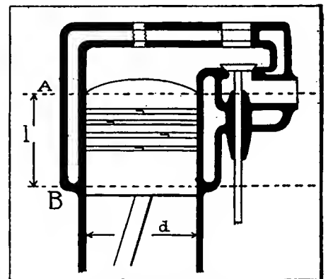
Fig. 2—Diagram illustrating meaning of piston displacement
